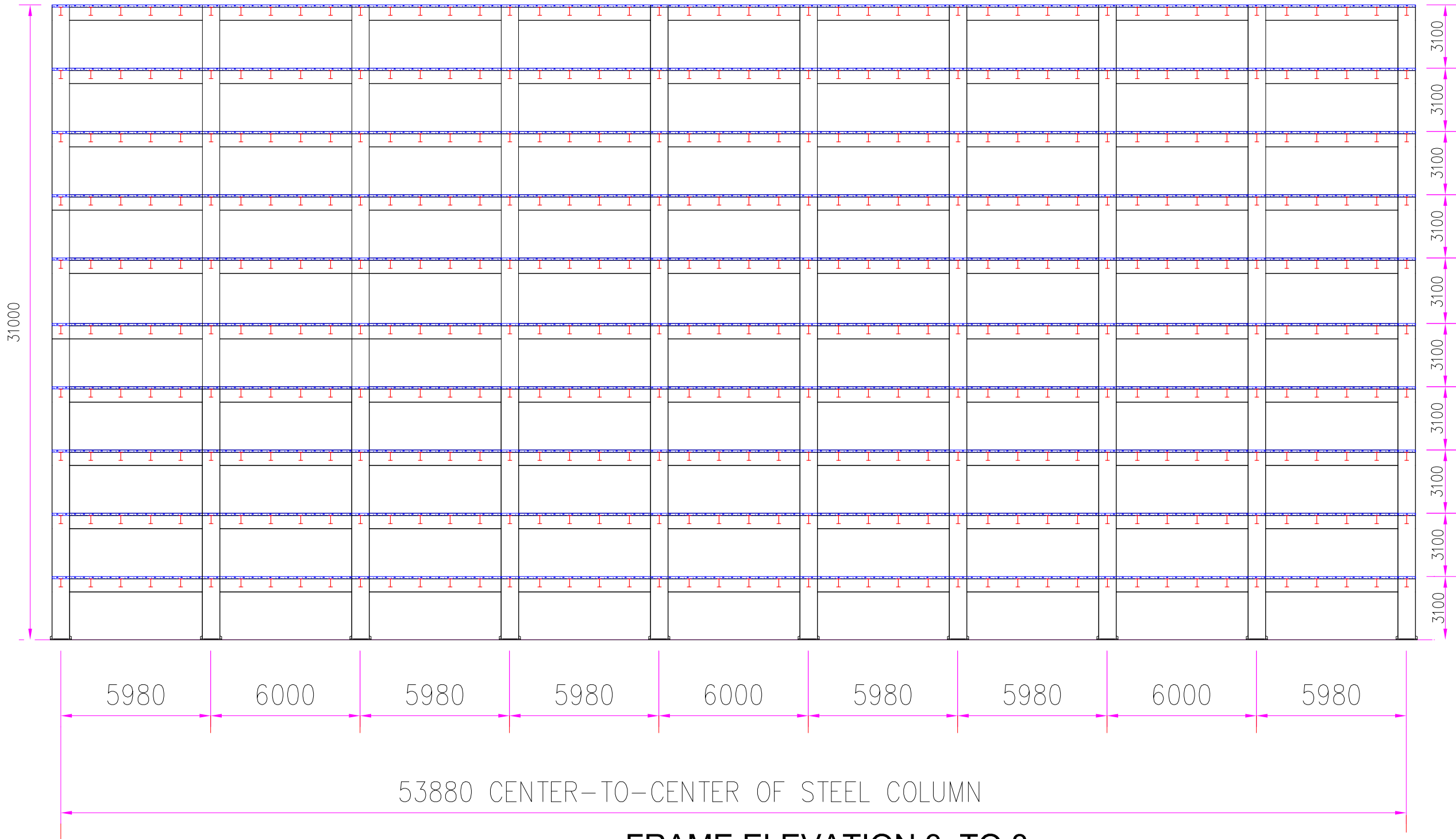
FRAME ELEVATION 3 TO 8
